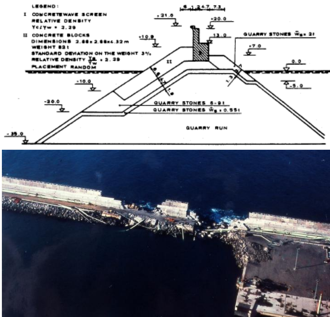
Figure 7 Bilbao breakwater cross section and photo of damage from the port side.
